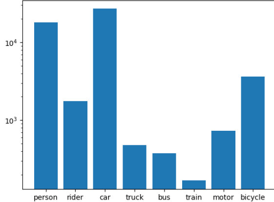
Fig. 2: Cityscapes dataset class histogram (logarithmic scale).
